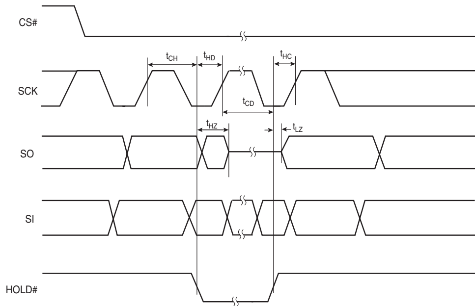
Figure 16.4 HOLD# Timing
