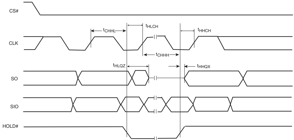
Figure 7.5 Hold Timing
