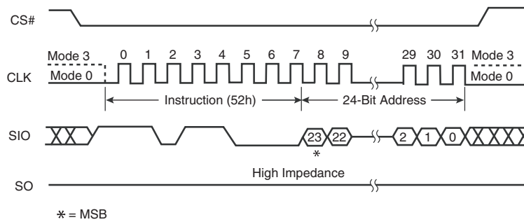
Figure 6.25 32 kB Block Erase Instruction Sequence Diagram
