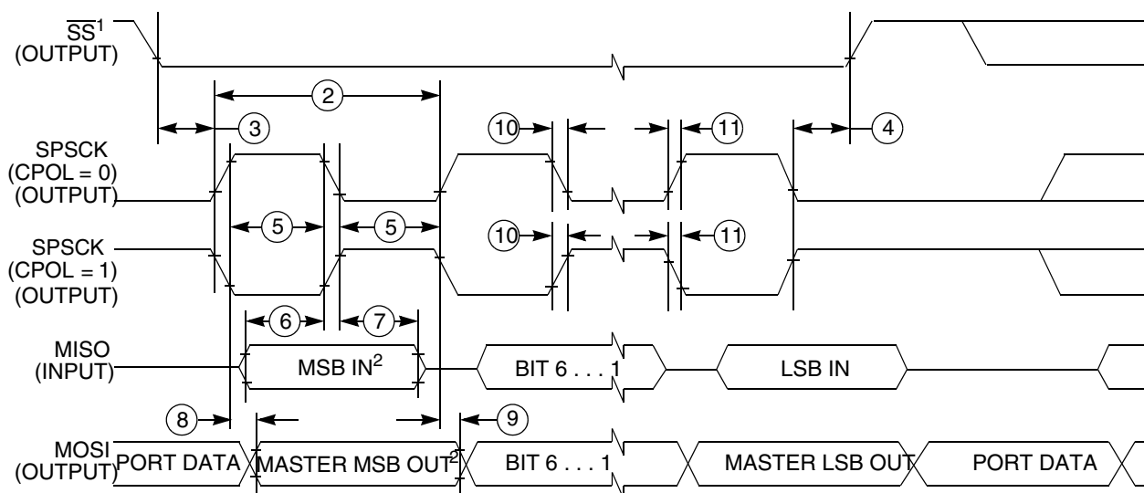
Figure 11. SPI master mode timing (CPHA = 1)
