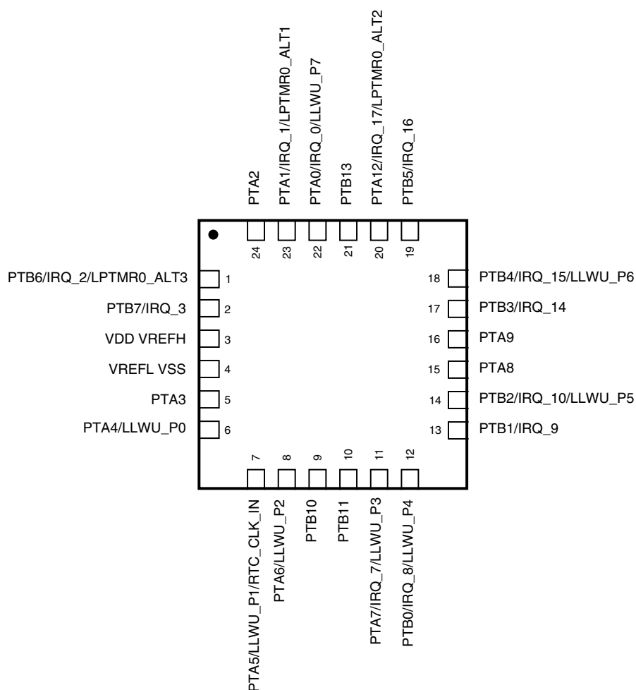
Figure 17. KL04 24-pin QFN pinout diagram
