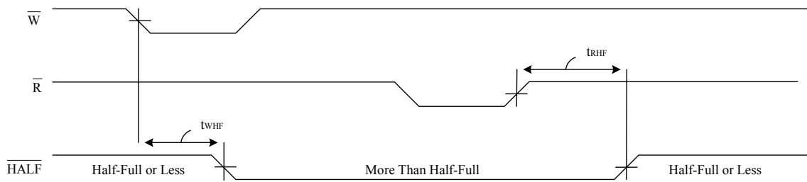
Diagram 8. Half-Full Flag Timing
