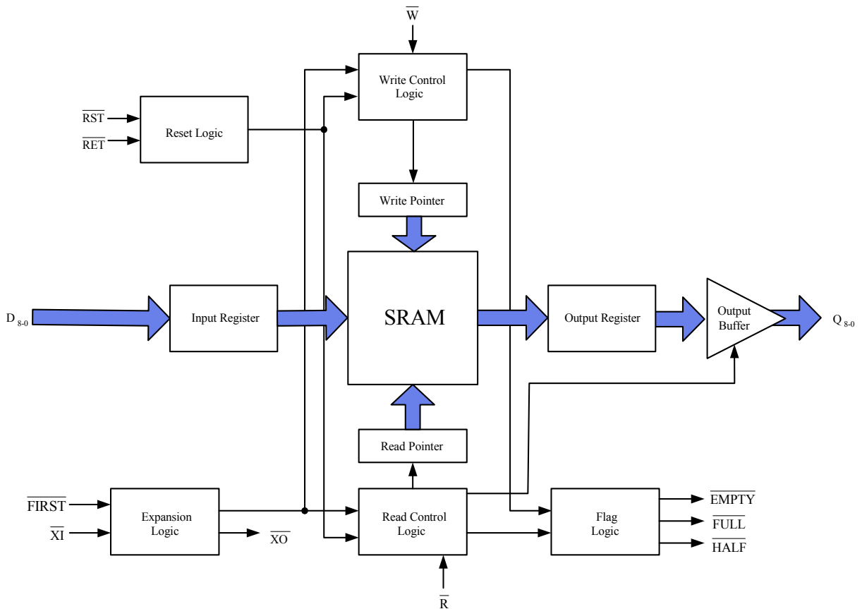
Block Diagram of Single Asynchronous Queue 8,192 x 9 / 4,096 x 9 / 2,048 x 9 / 1,024 x 9 / 512 x 9
