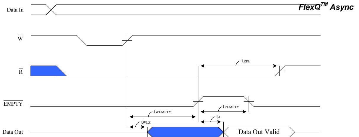
Diagram 11. Read Data Flow-Through Mode
