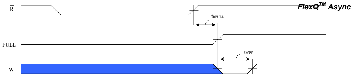
Diagram 7. Minimum Timing for a Full Flag Coincident Write Pulse
