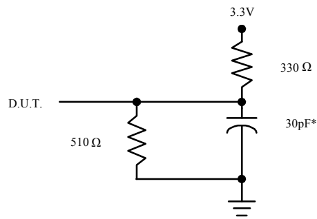
Figure 4. Output Load
