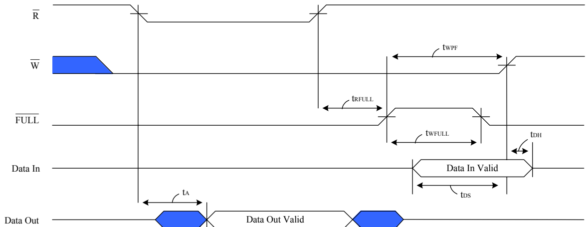
Diagram 12. Write Data Flow-Through Mode
