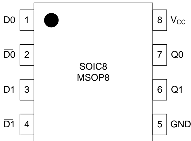
Figure 1 - Pin Configuration for SOIC8/MSOP8
