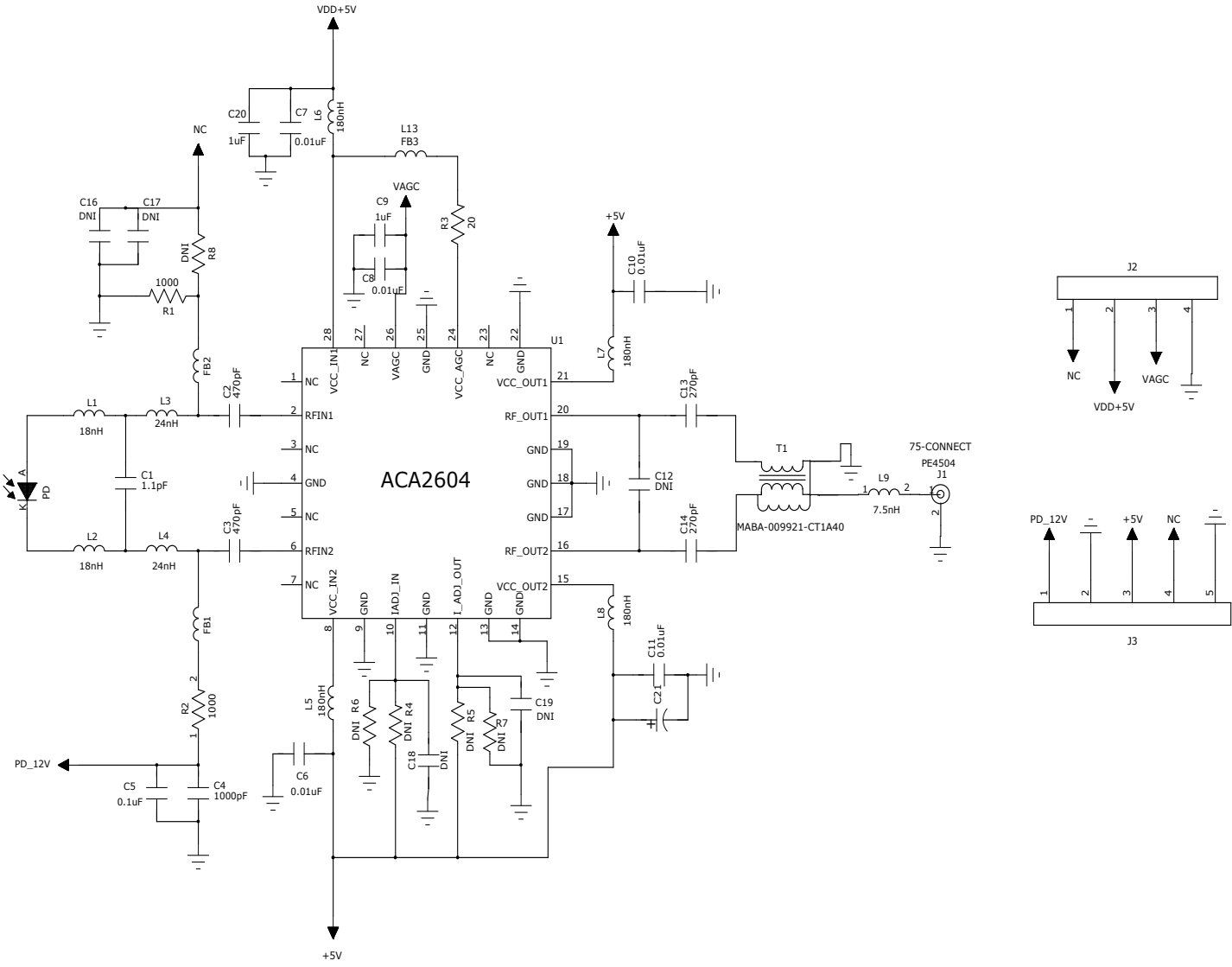
Figure 11: Application Circuit
