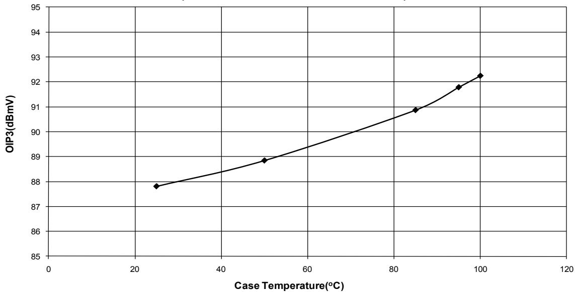
Figure 7: Output Third Order Intercept Point (OIP3) vs Temperature ( V_{dd} = +5\text{ Vdc} , F1 = 10\text{ MHz} , f2 = 11\text{ MHz} )
