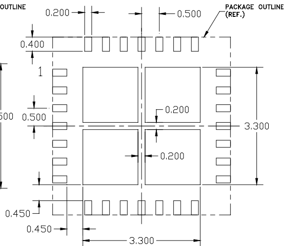
STENCIL APERTURE TOP (X-RAY) VIEW
