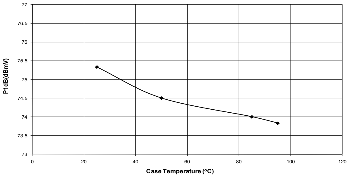
Figure 7: 1dB Gain Compression (P1dB) vs. Temperature ( V_{DD} = +5\text{ V} , F_1 = 10\text{ MHz} )
