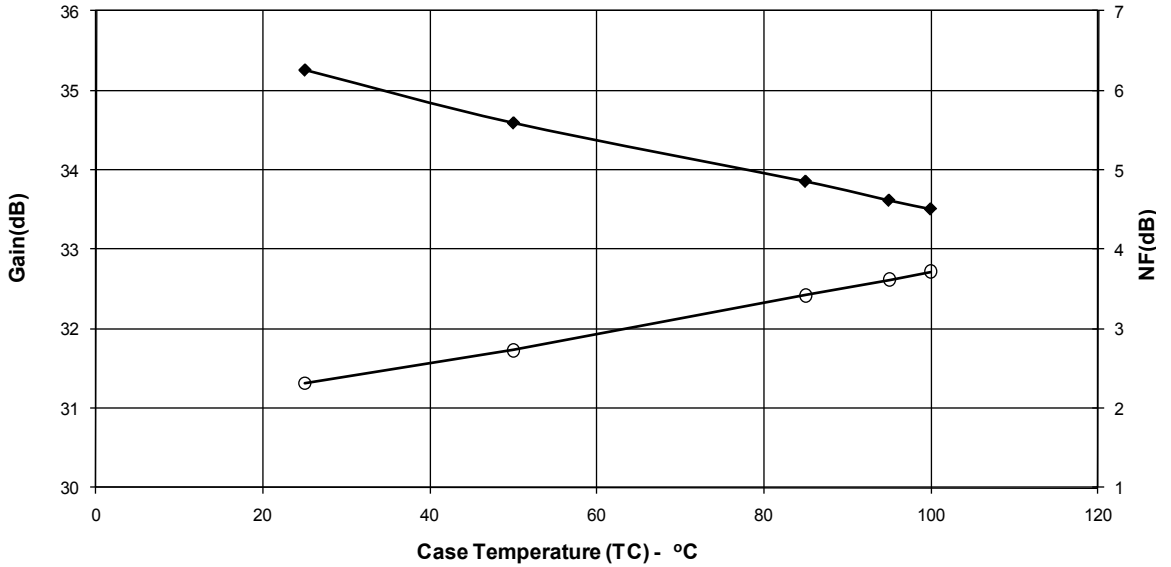
Figure 5: Gain & Noise Figure vs. Temperature (Vdd = +5V, F1 = 10 MHz)
