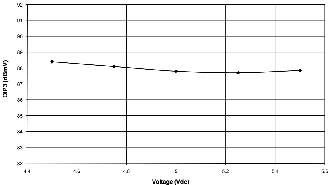
Figure 8: Output Third Order Intercept Point (OIP3) vs. Voltage ( T_c = 25\text{ °C} , F_1 = 10\text{ MHz} , F_2 = 11\text{ MHz} )
