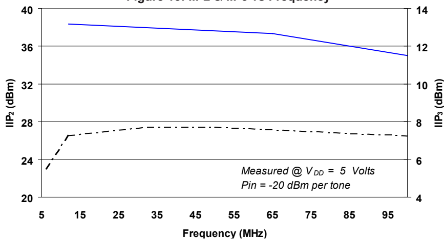
Figure 15: IIP2 &amp; IIP3 vs Frequency
