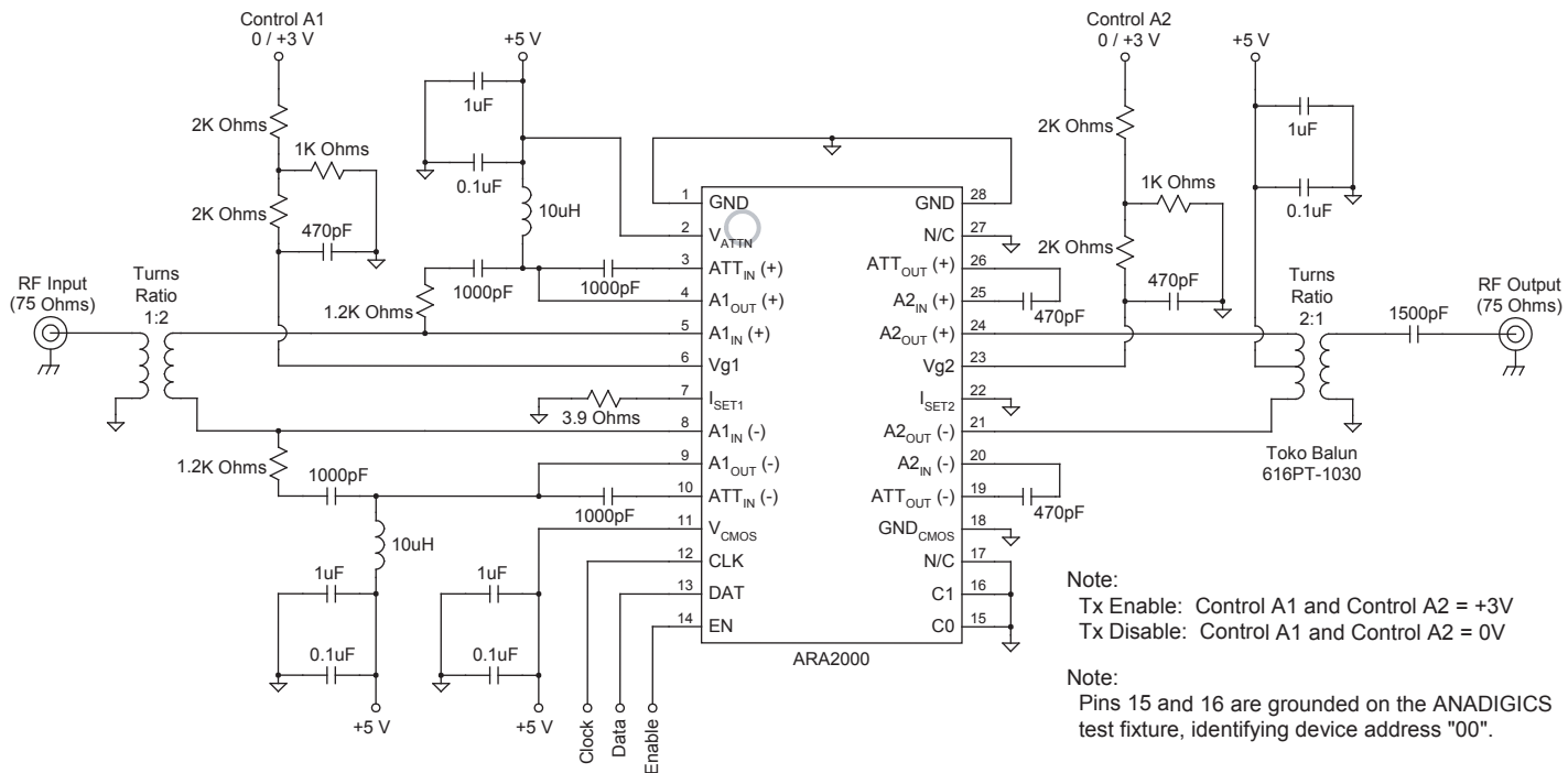
Figure 4: Test Circuit
