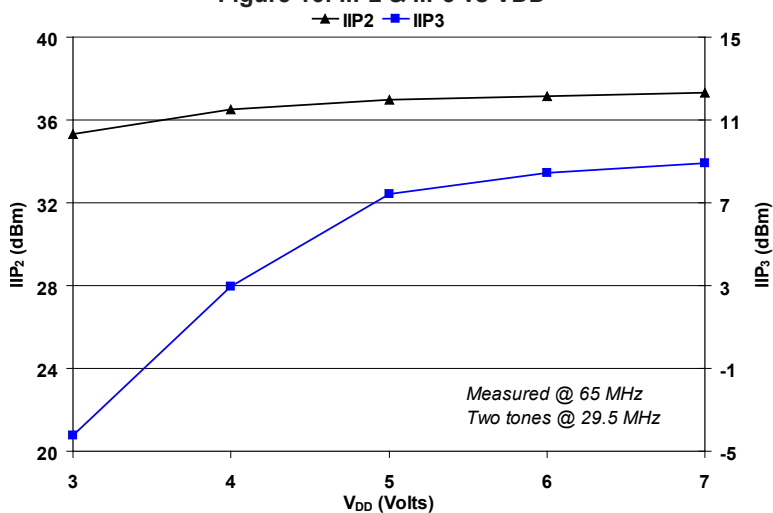
Figure 16: IIP2 &amp; IIP3 vs VDD
