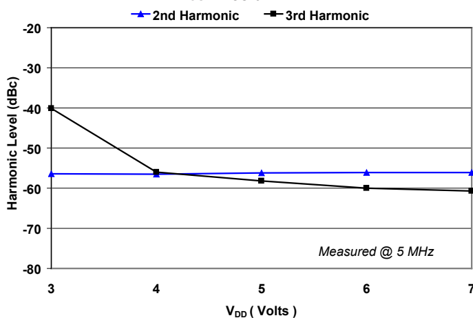
Figure 10: Harmonic Distortion vs VDD
