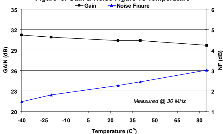
Figure 8: Gain &amp; Noise Figure vs Temperature
