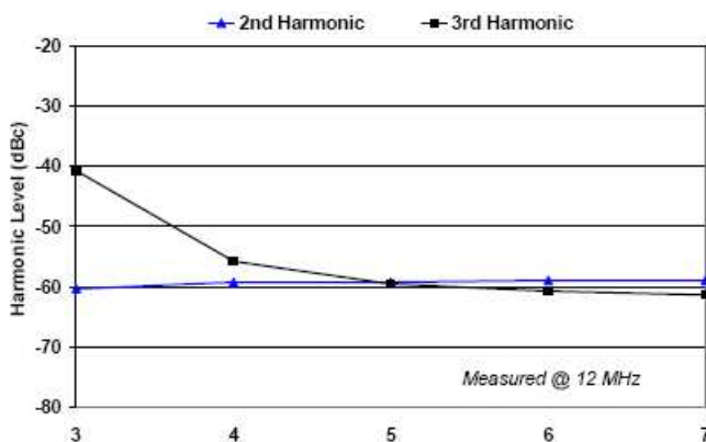
Figure 10: Harmonic Distortion vs V_{DD}
