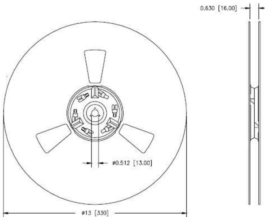
Figure 21: Reel Dimensions
