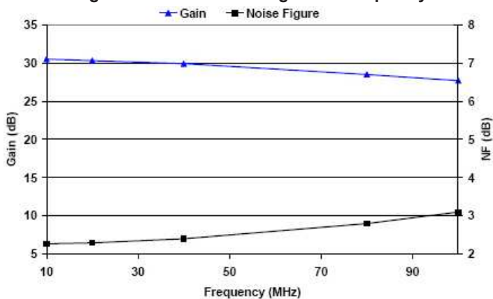
Figure 6: Gain &amp; Noise Figure vs Frequency
