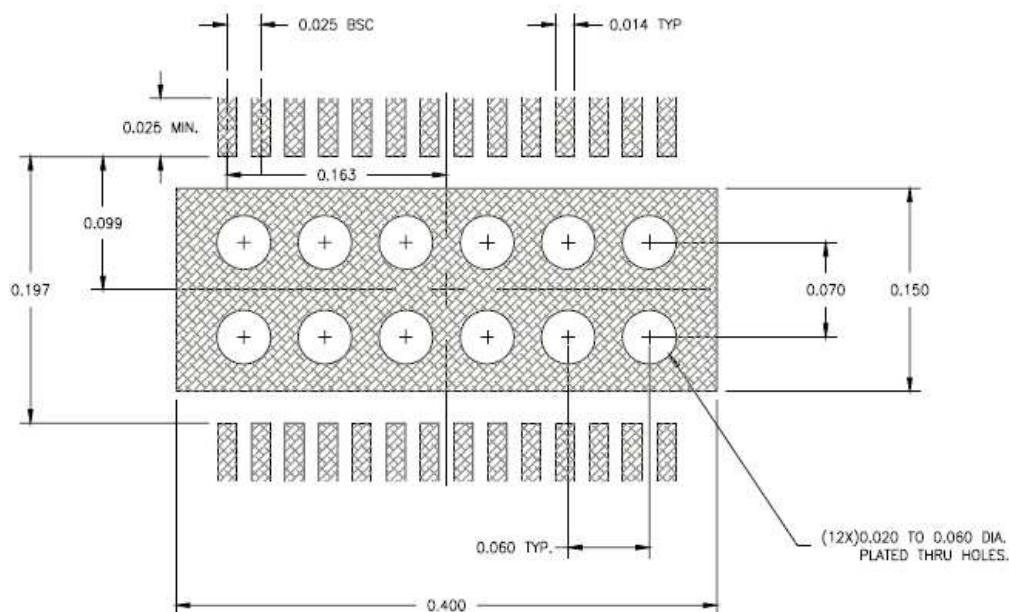
Figure 18: PC Board Layout
