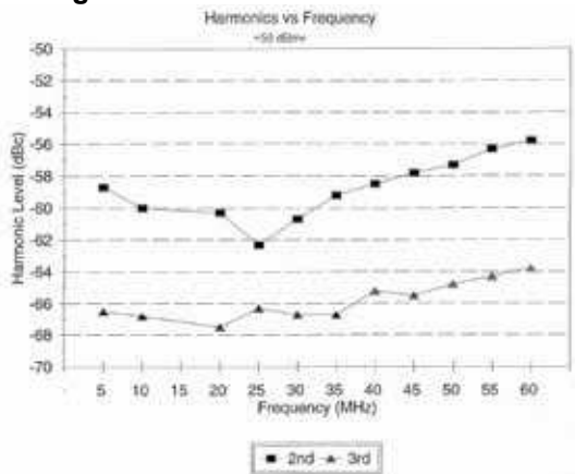
Figure 12: Harmonic Performance
