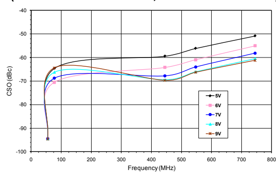
Figure 27: CSO vs Frequency and Voltage (110 Flat NTSC Channels; P OUT = +30 dBmV/ch)
