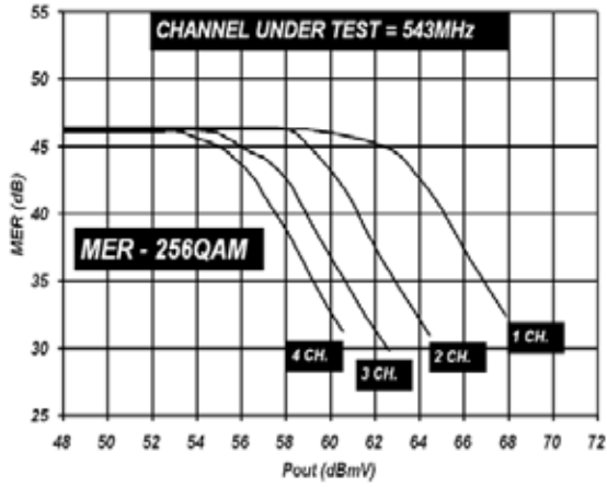
Figure 46: ADA10000 MER – 256 QAM @ 543 MHz
