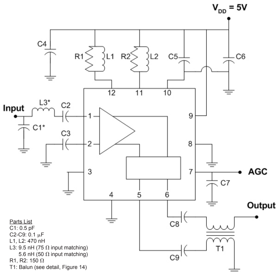
Figure 18: Test Circuit
