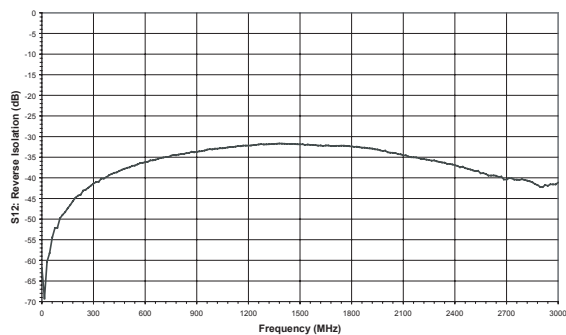
Figure 5: Reverse Isolation (S12) vs. Frequency ( T_C = +25^\circ\text{C} , V_{DD} = +5\text{ V} , V_{AGC} = +3\text{ V} )
