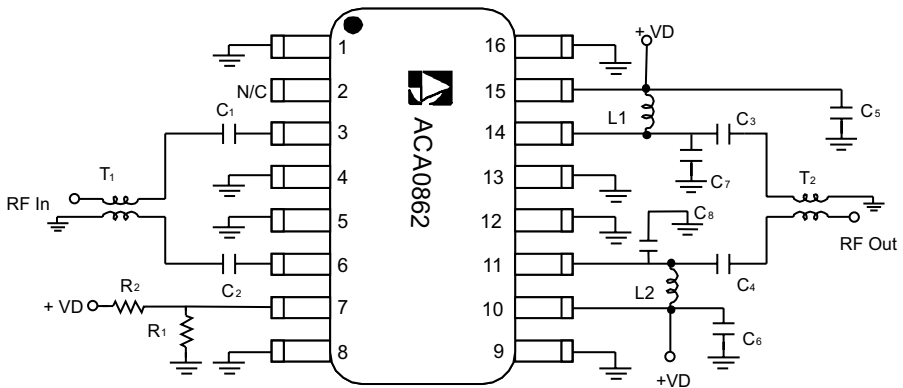
Figure 17: Test Circuit
