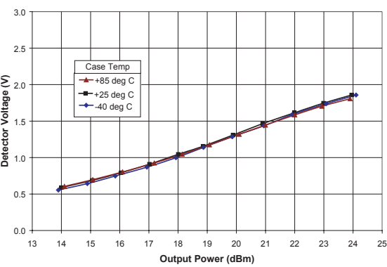
Figure 18: Effects of Case Temperature on Detector Voltage ( V_{CC} = +3.3\text{ V} , V_{BIAS} = +2.85\text{ V} , f = 2.6\text{ GHz} , 54 Mbps OFDM Modulation)
