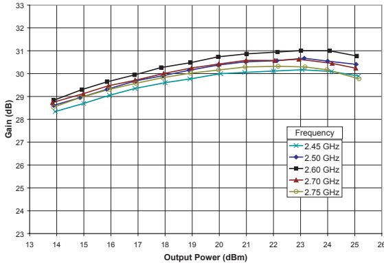
Figure 5: Gain vs. Output Power ( T_C = +25^\circ\text{C} , V_{CC} = +3.3\text{ V} , V_{BIAS} = +2.85\text{ V} , 54 Mbps OFDM Modulation)
