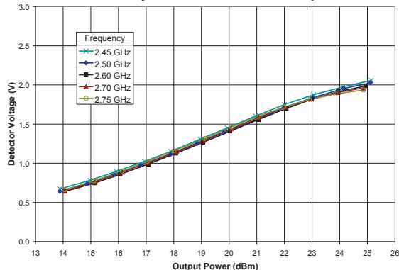
Figure 13: Detector Voltage vs. Output Power ( T_C = +25\text{ }^\circ\text{C} , V_{CC} = +3.3\text{ V} , V_{BIAS} = +2.85\text{ V} , 54 Mbps OFDM Modulation)
