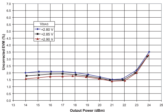
Figure 12: Effects of Bias Voltage (V BIAS ) on EVM ( T_C = +25\text{ }^\circ\text{C} , V_{CC} = +3.3\text{ V} , f = 2.6\text{ GHz} , 54 Mbps OFDM Modulation, system EVM approx. 0.8 %)
