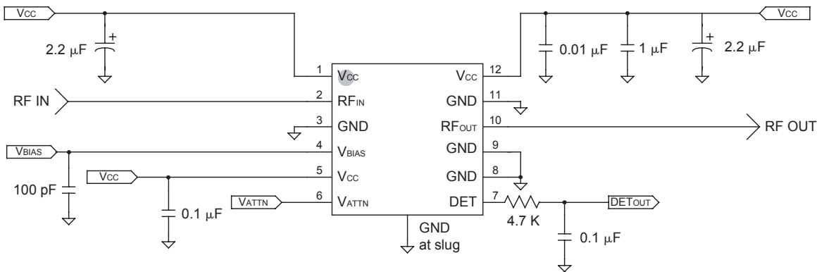
Figure 19: Application Circuit
