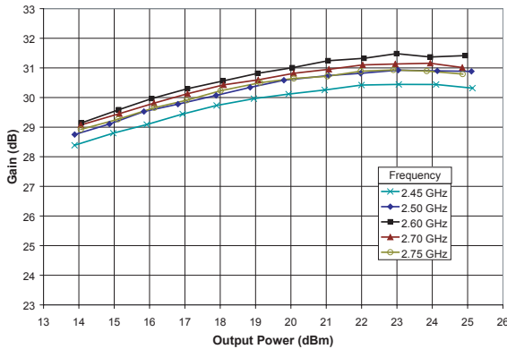
Figure 7: Gain vs. Output Power ( T_C = +25^\circ\text{C} , V_{CC} = +4.2\text{ V} , V_{BIAS} = +2.85\text{ V} , 54 Mbps OFDM Modulation)
