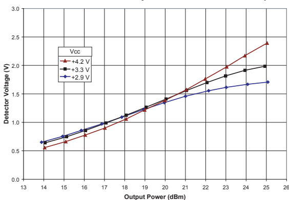
Figure 14: Effects of Supply Voltage (V CC ) on Detector Voltage ( T_C = +25\text{ }^\circ\text{C} , V_{BIAS} = +2.85\text{ V} , f = 2.6\text{ GHz} , 54 Mbps OFDM Modulation)
