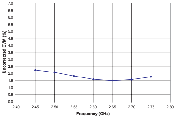
Figure 10: Uncorrected EVM vs. Frequency ( T_C = +25\text{ }^\circ\text{C} , V_{CC} = +3.3\text{ V} , V_{BIAS} = +2.85\text{ V} , 54 Mbps OFDM Modulation, system EVM approx. 0.8 %)
