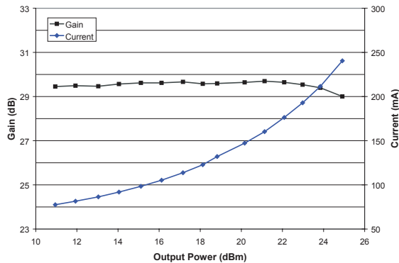
Figure 5: Gain and Current Consumption vs Output Power (T A = +25 °C, V CC = +3.3 V, V REF = +2.85 V, f = 2472 MHz, 54 Mbps 802.11g)
