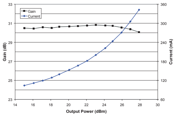
Figure 6: Gain and Current Consumption vs. Output Power (T A = +25 °C, V CC = +5 V, V REF = +2.85 V, f = 2472 MHz, 54 Mbps 802.11g)
