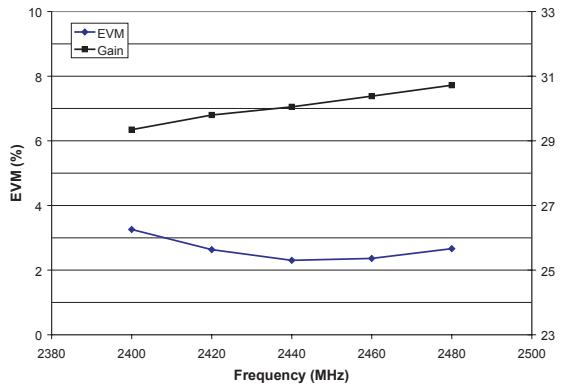
Figure 4: EVM and Gain vs Frequency (T A = +25 °C, V CC = +5 V, V REF = +2.85 V, P OUT = +25 dBm, 54 Mbps 802.11g)
