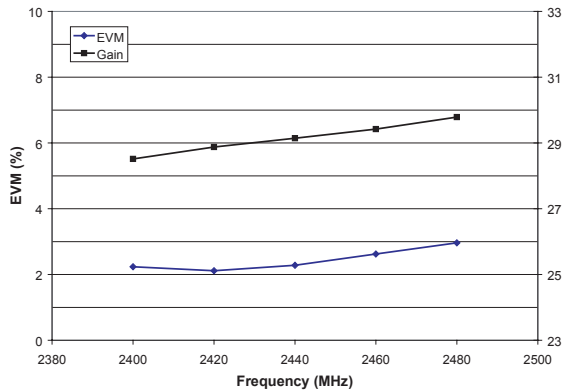
Figure 3: EVM and Gain vs Frequency (T A = +25 °C, V CC = +3.3 V, V REF = +2.85 V, P OUT = +21 dBm, 54 Mbps 802.11g)
