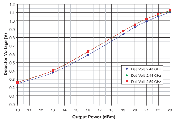
Figure 17: Detector Voltage vs. Output Power Across Freq ( V_{CC} = +3.3 V, T_C = 25^\circ\text{C} , 2 K \Omega Load) 2.4 GHz 802.11b Gaussian Filtering (BT = 0.45), 1 Mbps
