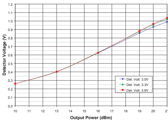
Figure 19: Detector Voltage vs. Output Power Across Supply Voltage (Freq = 2.45 GHz, T_C = 25^\circ\text{C} , 2 K \Omega Load) 2.4 GHz 802.11b Gaussian Filtering (BT = 0.45), 1 Mbps
