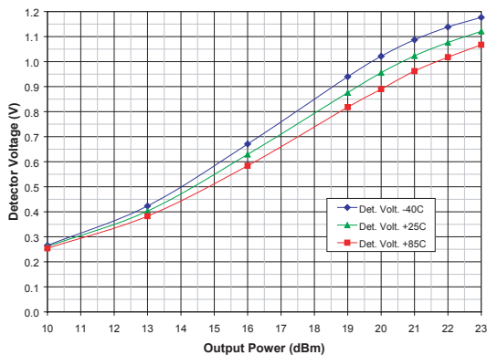
Figure 18: Detector Voltage vs. Output Power Across Temp (Freq = 2.45 GHz, V_{CC} = +3.3 V, 2 K \Omega Load) 2.4 GHz 802.11b Gaussian Filtering (BT = 0.45), 1 Mbps
