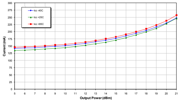
Figure 12: Tx Path Icc vs. Output Power Across Temperature (Freq = 5.5 GHz, Vcc = +3.3 V 802.11a, 54 Mbps OFDM)
