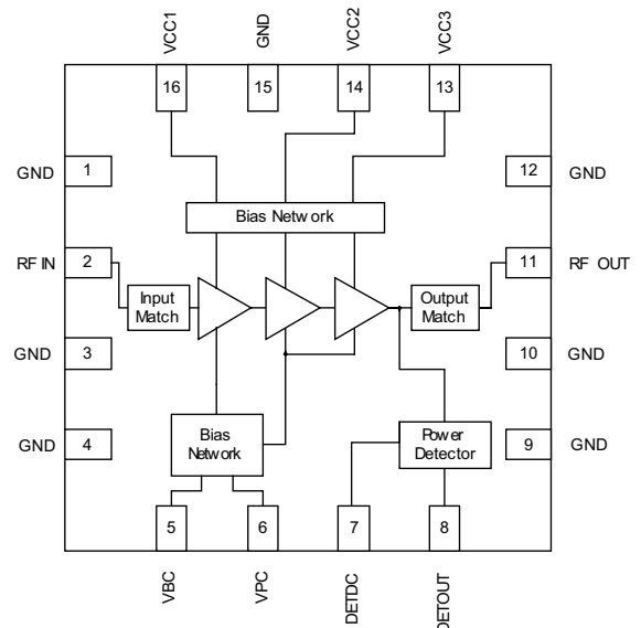
Figure 1: Block Diagram and Pinout
