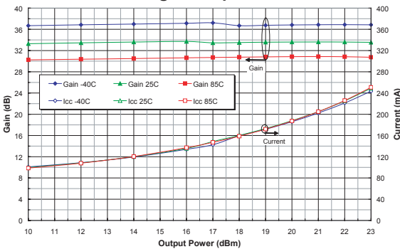
Figure 29: Gain and I_{CC} vs. Output Power Across Temp (Frequency = 2.45 GHz, V_{CC} = +4.2 V ) 802.11g 54 Mbps OFDM
