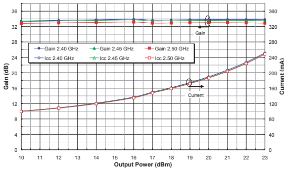
Figure 27: Gain and I_{CC} vs. Output Power Across Frequency ( V_{CC} = +4.2 V , T_C = +25^\circ C ) 802.11g 54 Mbps OFDM
