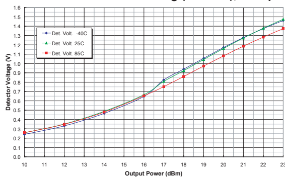
Figure 18: Detector Voltage vs. Output Power Across Temp (Frequency = 2.45 GHz, V CC = +3.3V) 802.11b Root Cosine Filtering ( \alpha = 0.50 ), 1 Mbps
