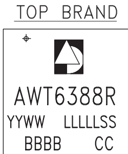
Figure 4: M20 Package Outline - 10 Pin 4 mm x 4 mm x 1 mm Surface Mount Module
