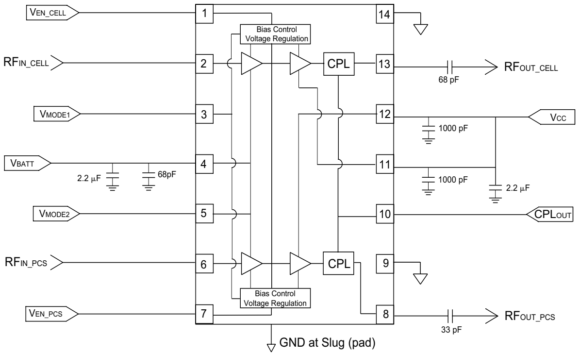
Figure 4: Application Circuit
