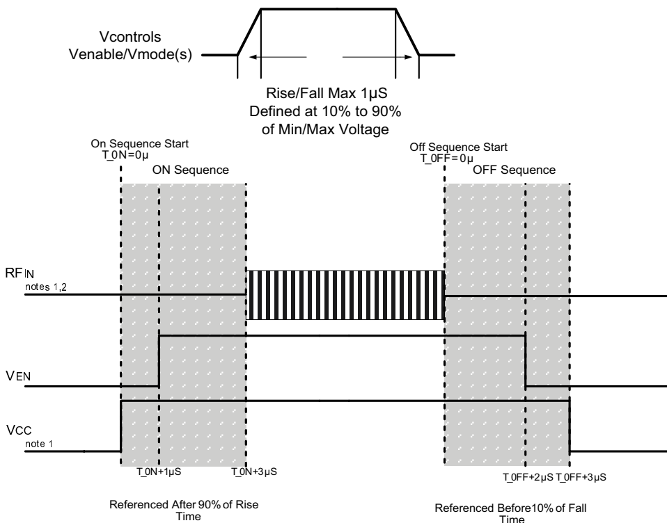
Figure 3: Recommended ON/OFF Timing Sequence
