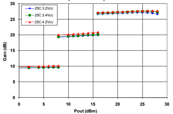
Figure 4: LTE Gain (dB) over Voltage ( T_c = 25\text{ }^\circ\text{C} )
