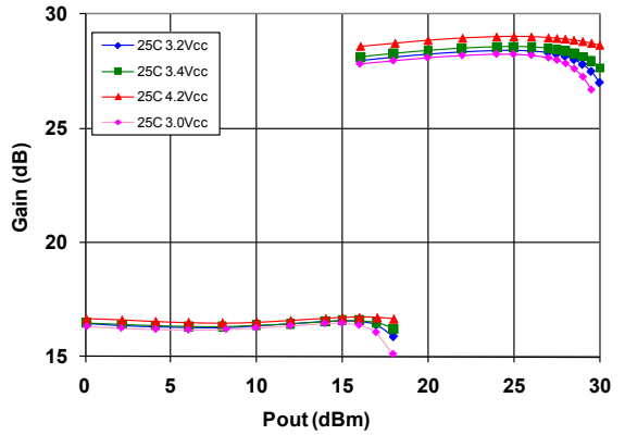
Figure 4: WCDMA Gain (dB) over Voltage ( T_c = 25\text{ °C} )
