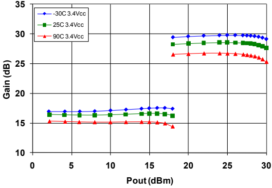
Figure 3: WCDMA Gain (dB) over Temperature ( V_{BATT} = V_{CC} = 3.4\text{ V} )
