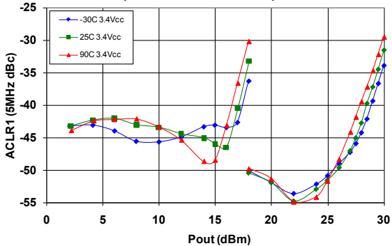
Figure 7: WCDMA ACLR1 (dBc) over Temperature ( V_{BATT} = V_{CC} = 3.4\text{ V} )
