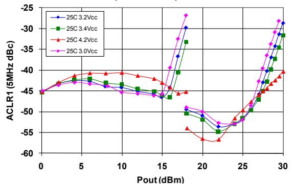
Figure 8: WCDMA ACLR1 (dBc) over Voltage ( T_c = 25\text{ °C} )
