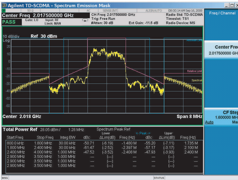
Fig 6: Spectrum Emission Mask @ 1.9GHz (Freq = 2017.5 MHz, P OUT = 28 dBm, V CC = 3.4 V, T c = 25 °C)
