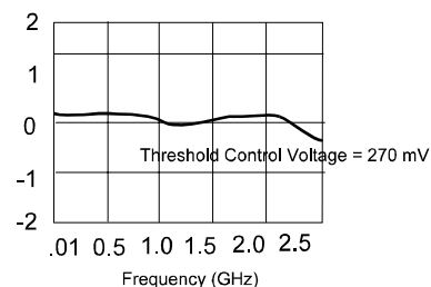
Input Power Flatness (dBm)
