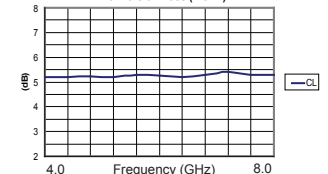
Conversion Loss (1 GHz)
