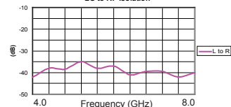
LO to RF Isolation
