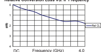
Relative Conversion Loss VS. IF Frequency
