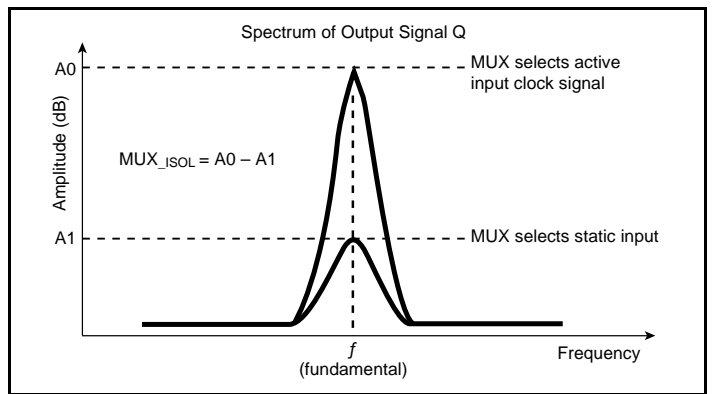
MUX Isolation
