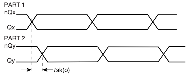
PART-TO-PART SKEW
