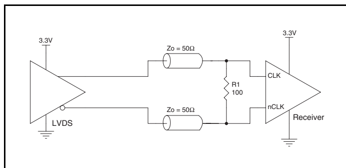
Figure 3D. HiPerClockS CLK/ \overline{\text{CLK}} Input Driven by a 3.3V LVDS Driver
