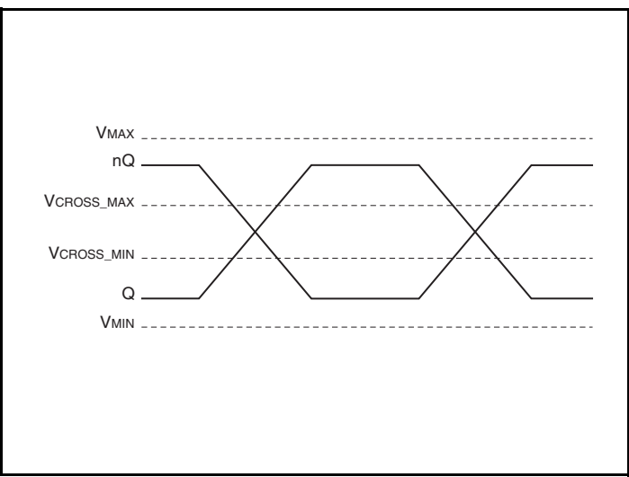
Single-ended Measurement Points for Absolute Cross Point and Swing
