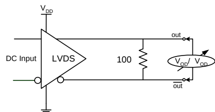
V_{OD} SETUP
