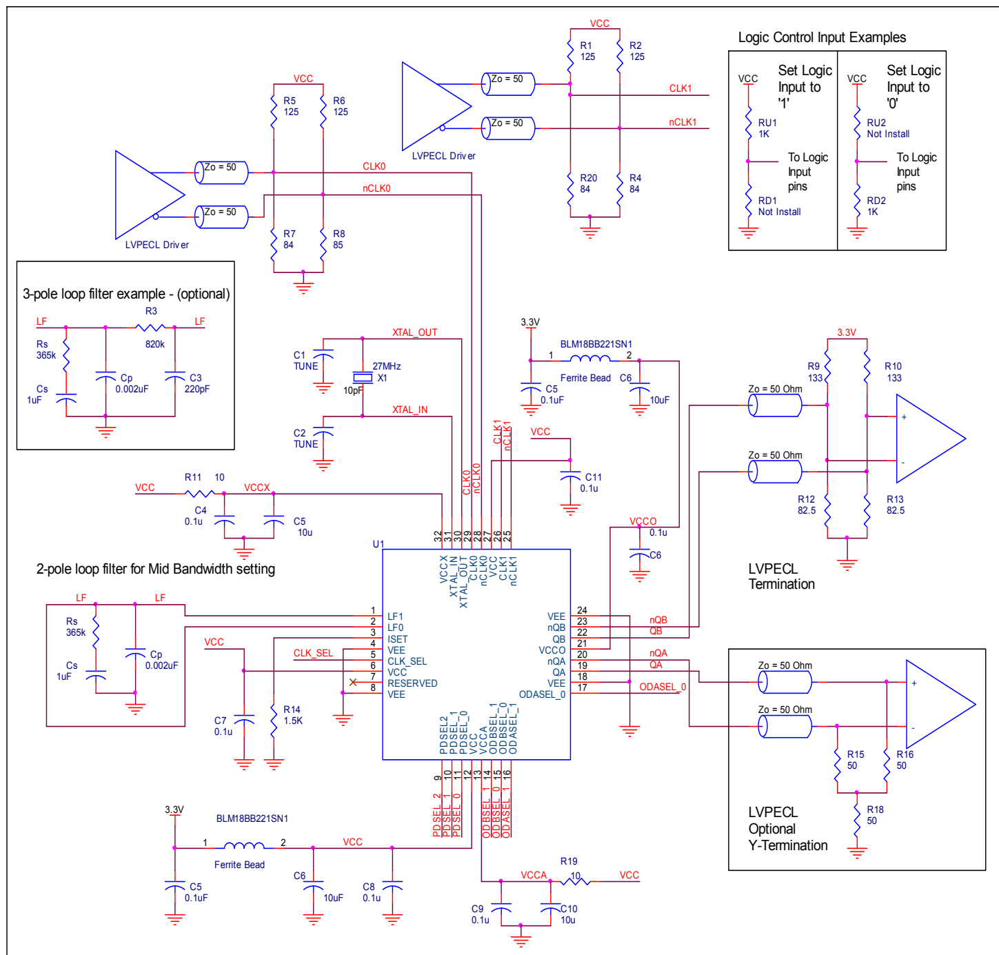
Figure 5. ICS813N252I-02 Schematic Example
