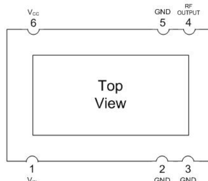
Figure 1: Pin Assignment
