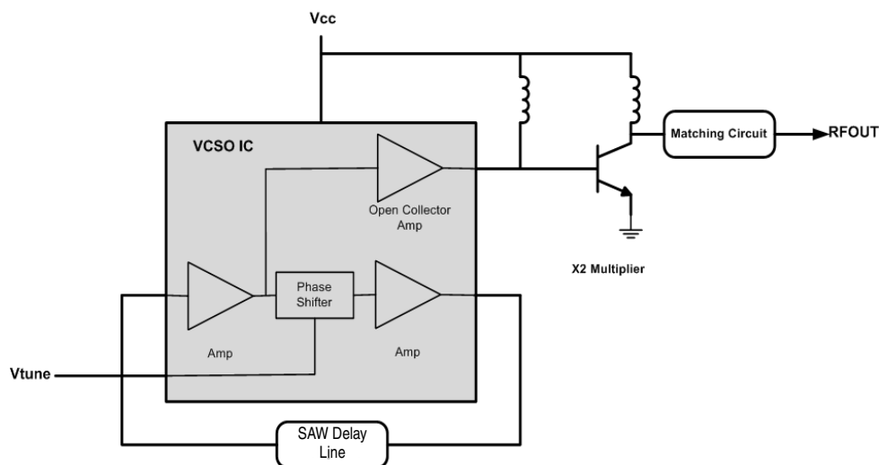
Figure 2: Block Diagram
