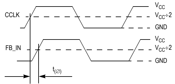
Figure 14. Propagation Delay ( t_0 ), status phase offset Test Reference
