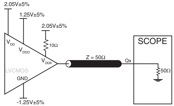
3.3V/2.5V OUTPUT LOAD AC TEST CIRCUIT
