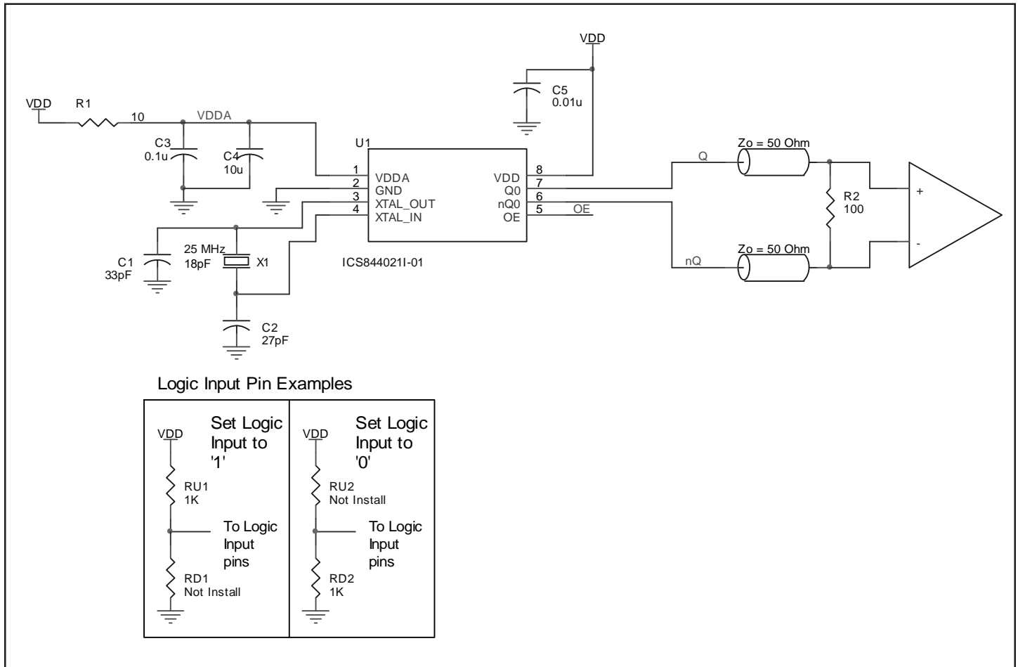
FIGURE 5. ICS844021I-01 SCHEMATIC LAYOUT
