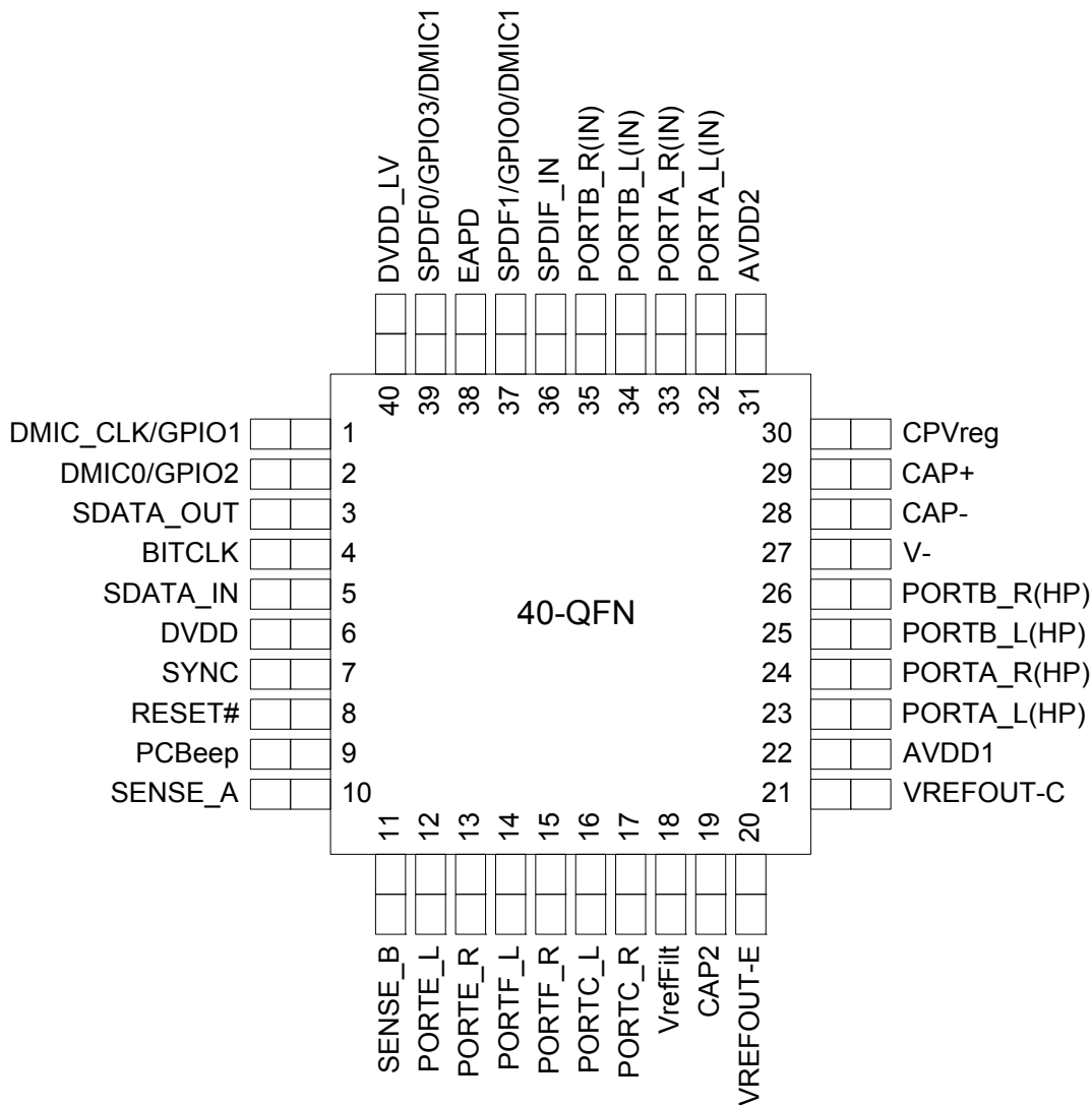
Figure 12. 40-Pin Pinout
