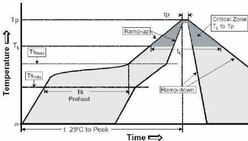
Figure 23. Reflow Profile
