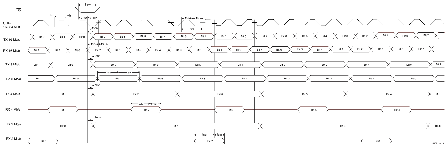
Figure 17. ST-BUS® Timing
