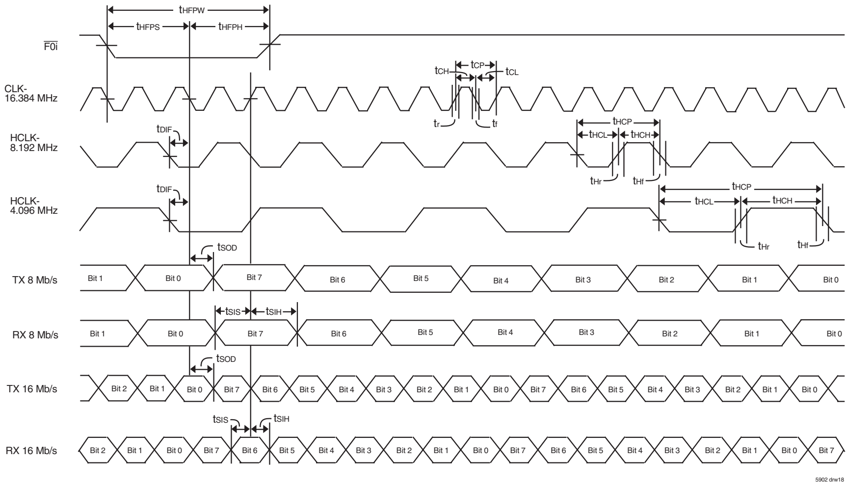
Figure 16. WFPS Timing
