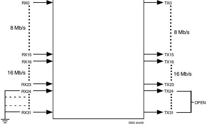
Figure 5. Split Mode
