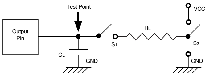
Figure 9. Output Load
