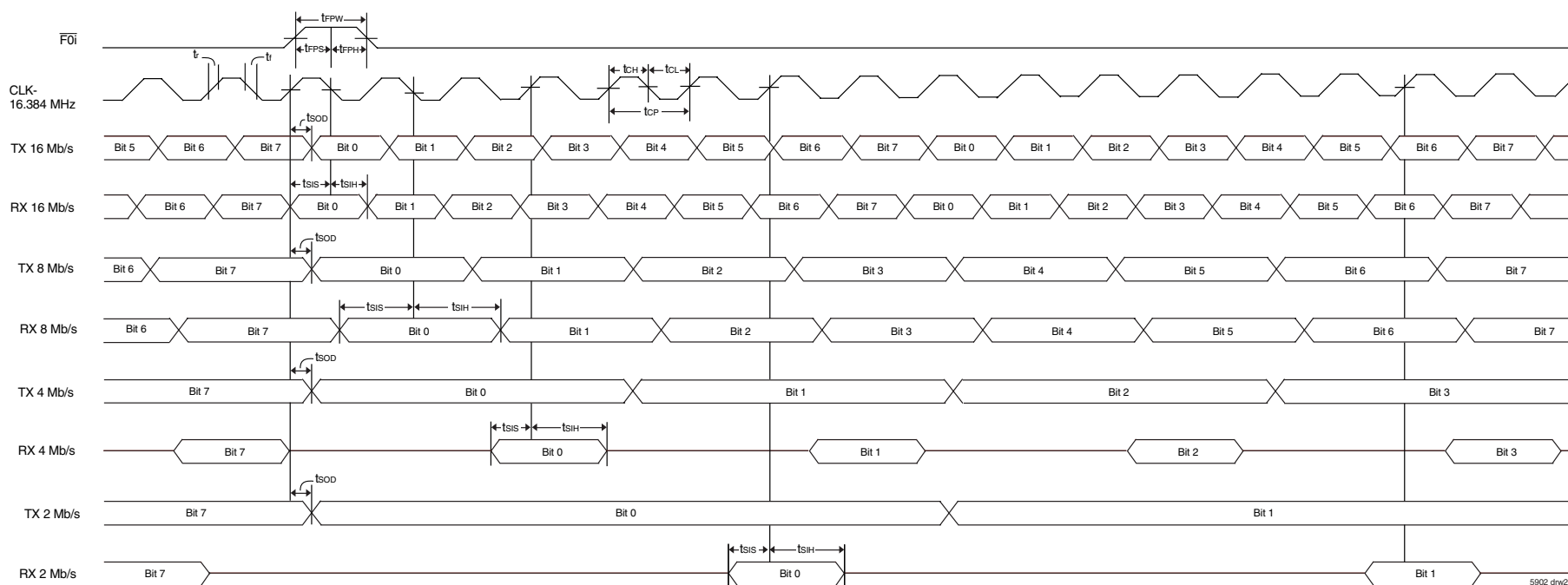
Figure 18. GCI Timing
