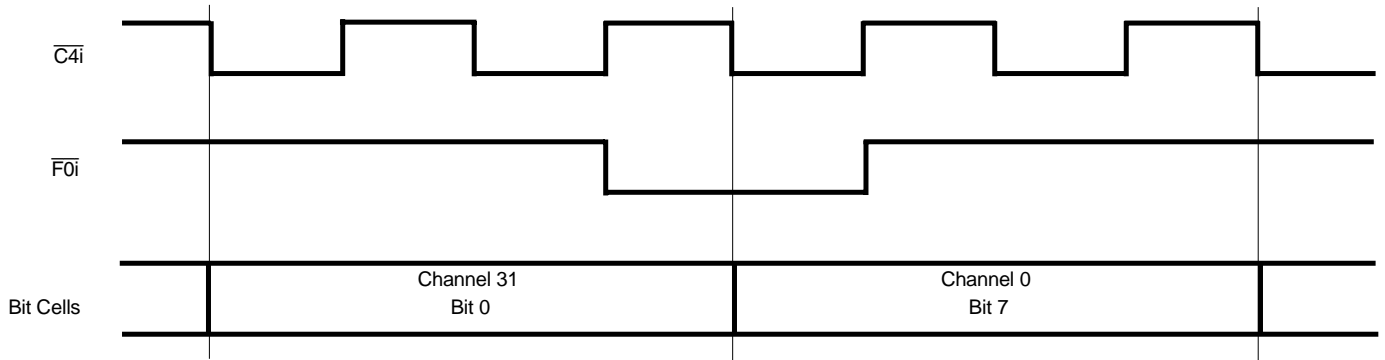
Figure 5. Frame Alignment
