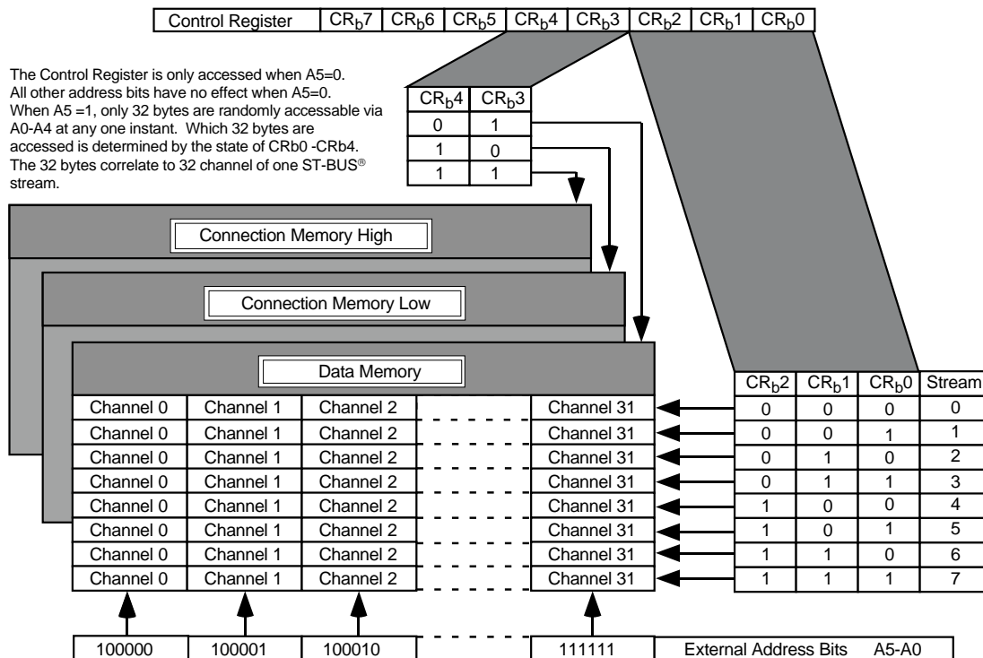
Figure 3. Address Mapping
