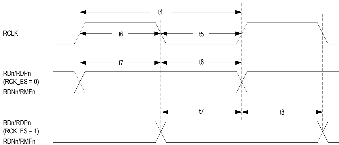
Figure-52 Receive Clock Timing Diagram
