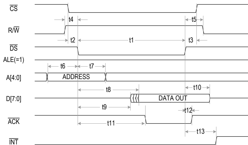
Figure-21 Non-Multiplexed Motorola Mode Read Timing
