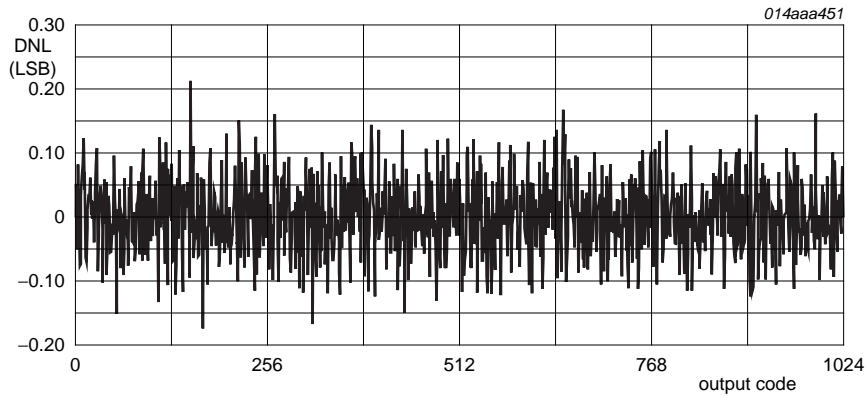
Fig 12. Differential Non-Linearity (DNL)
