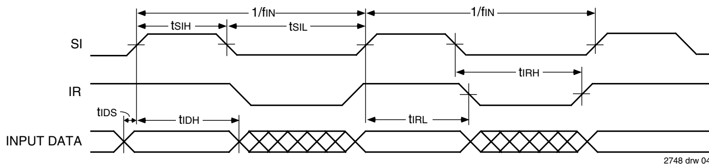
Figure 2. Input Timing
