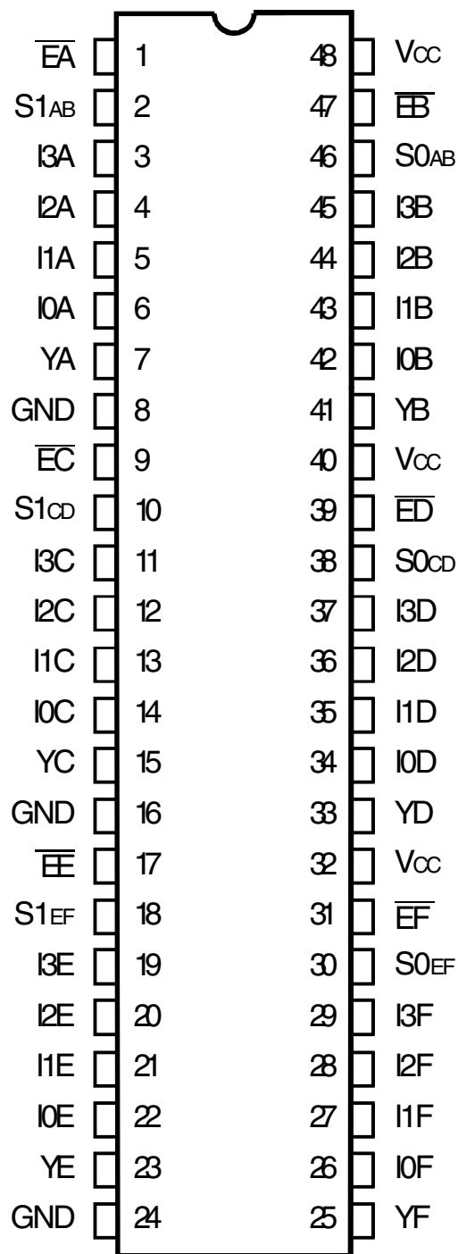
QVSOP TOP VIEW
