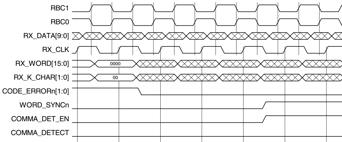
Figure 10 • Receive Error
