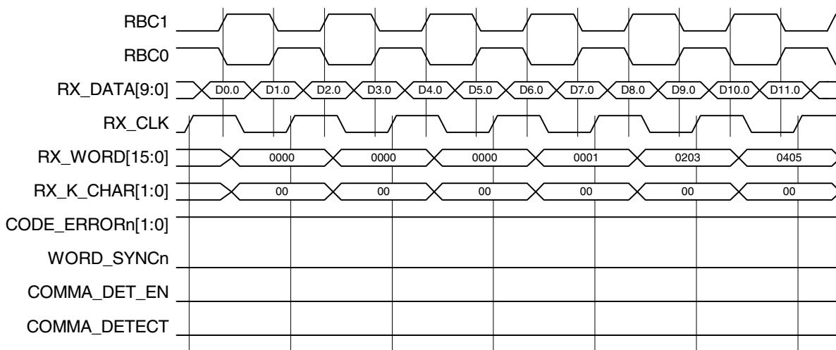
Figure 9 • Normal Receive
