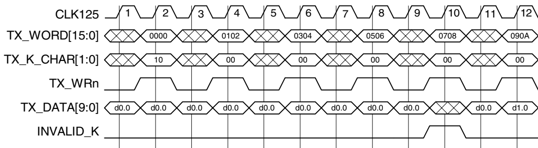
Figure 8 • Invalid Command
