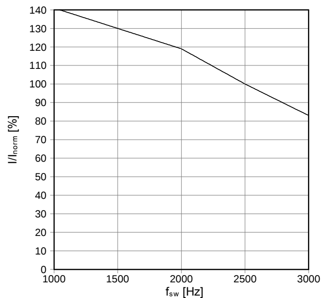
f sw - derating curve IGBT (motor) cos(φ) = 0,87 T cool medium = 25°C
