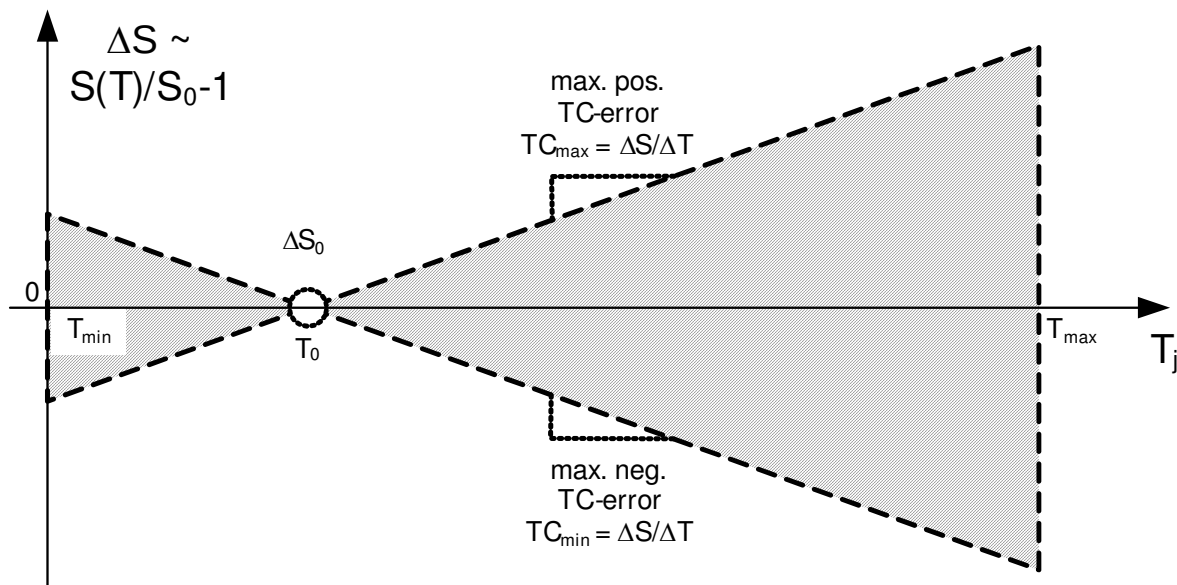
Figure 4 Sensitivity drift
