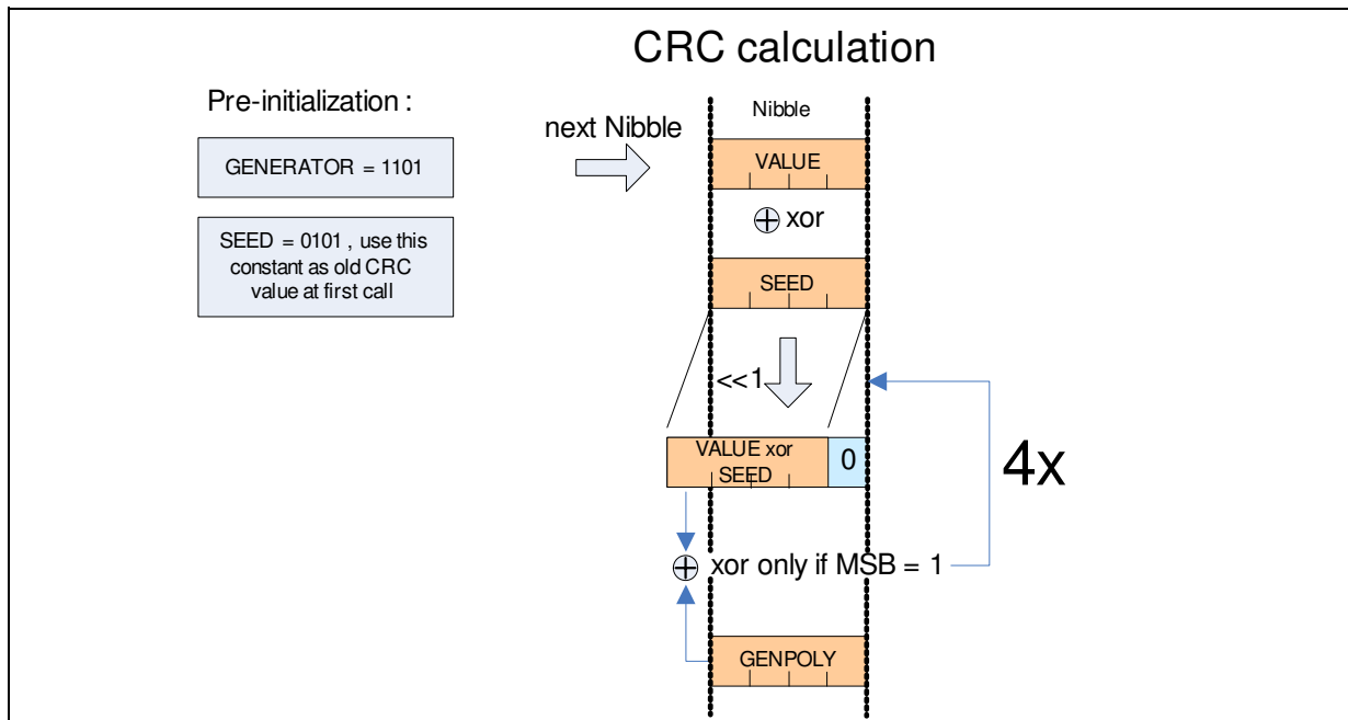
Figure 17 CRC Calculation
